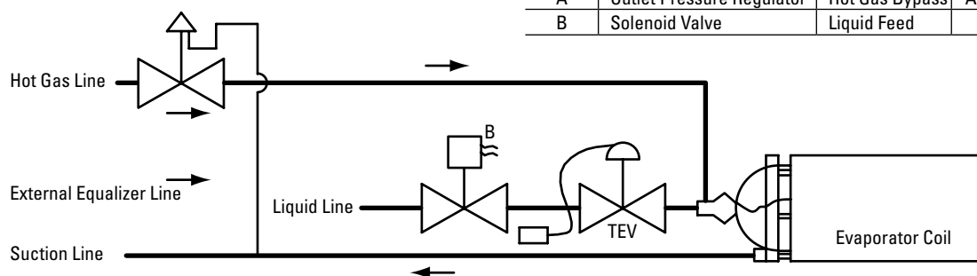
Figure 4 — Hot gas bypass to entrance of evaporator. See page 62 for symbols legend.
